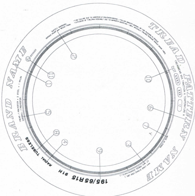
LOWER MOLD
